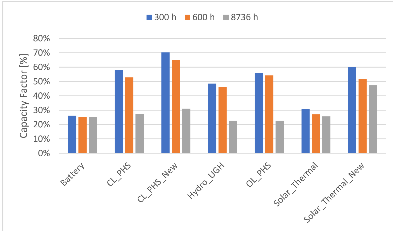
Technology capacity factors at peak hours of net demand
