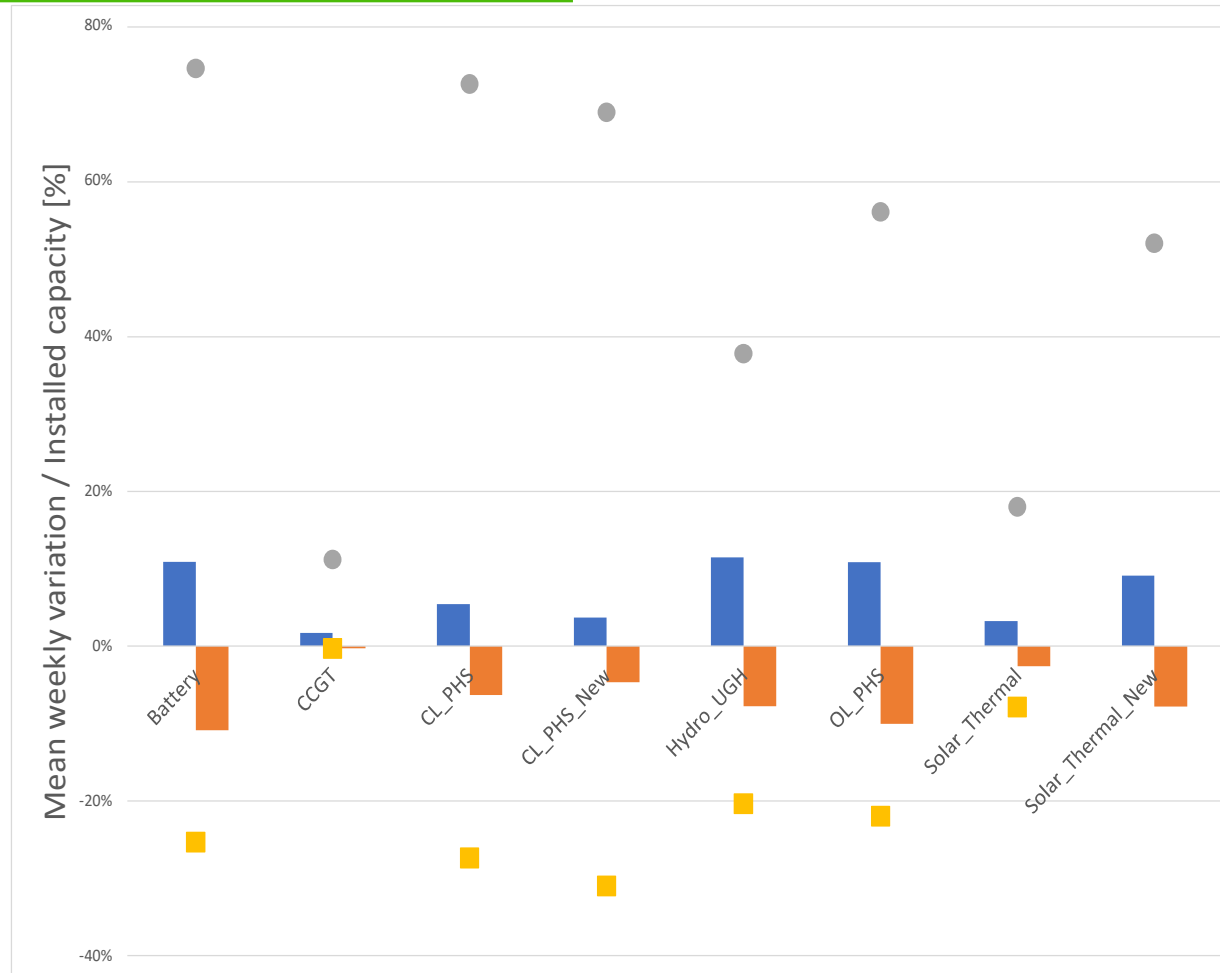
Mean weekly variation of each technology with respect to its installed capacity
