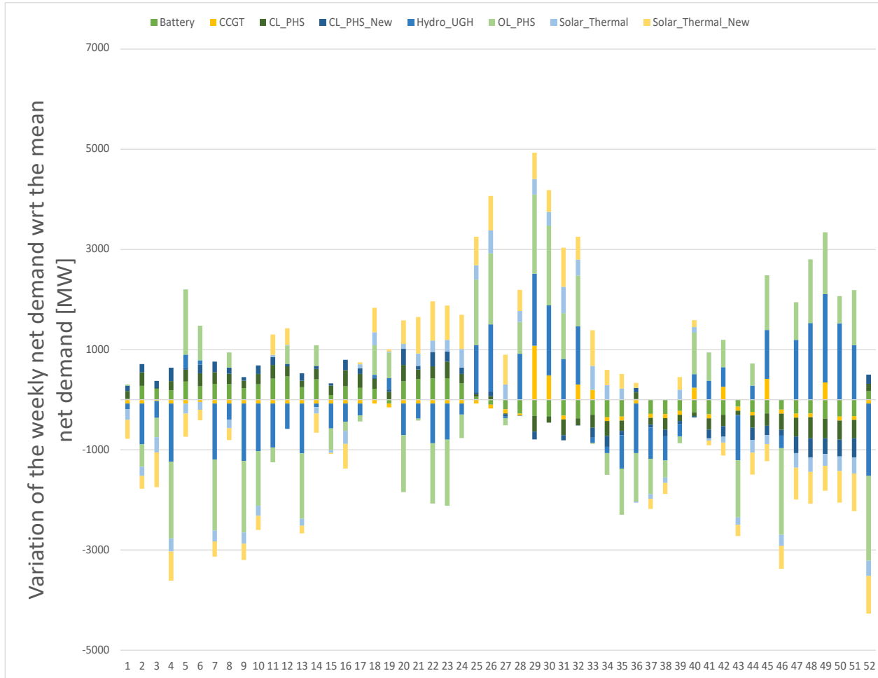
Contribution of each flexible technology to the variation of the weekly net demand with respect to the mean net demand
